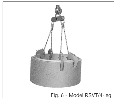
Fig. 6 - Model RSVT/4-leg
